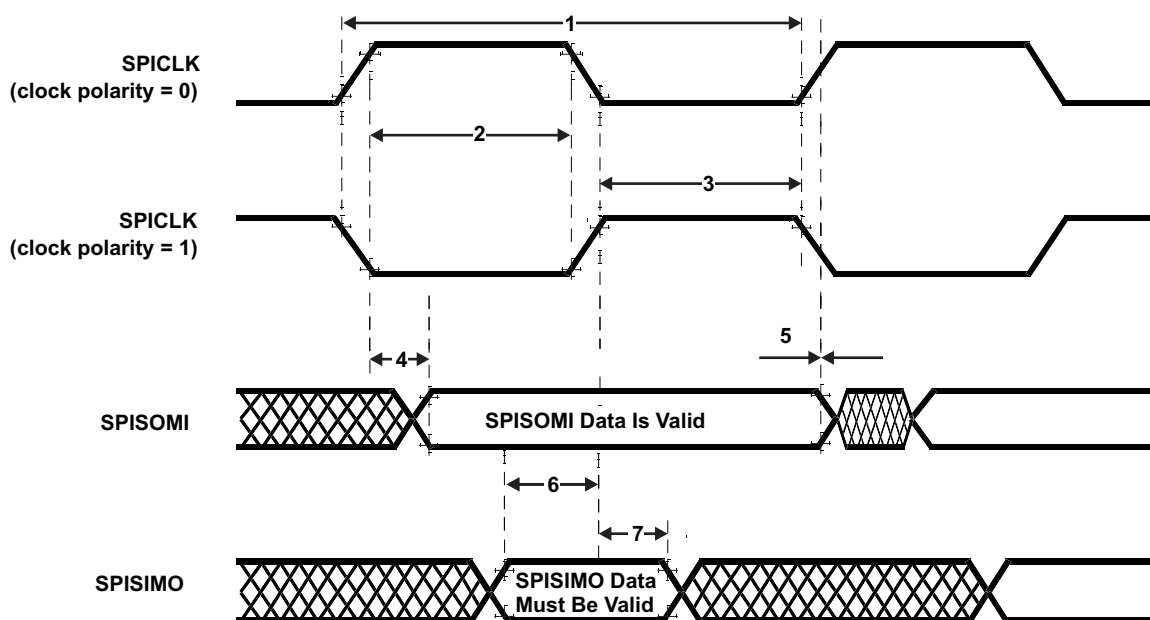
Figure 7-23. SPI Slave Mode External Timing (CLOCK PHASE = 0)
