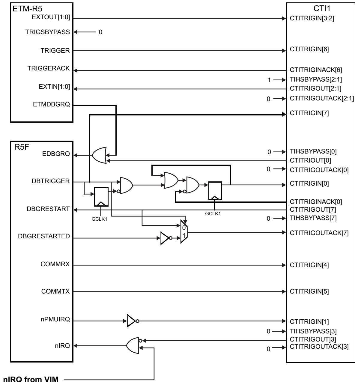
Figure 6-25. CTI1 Mapping
