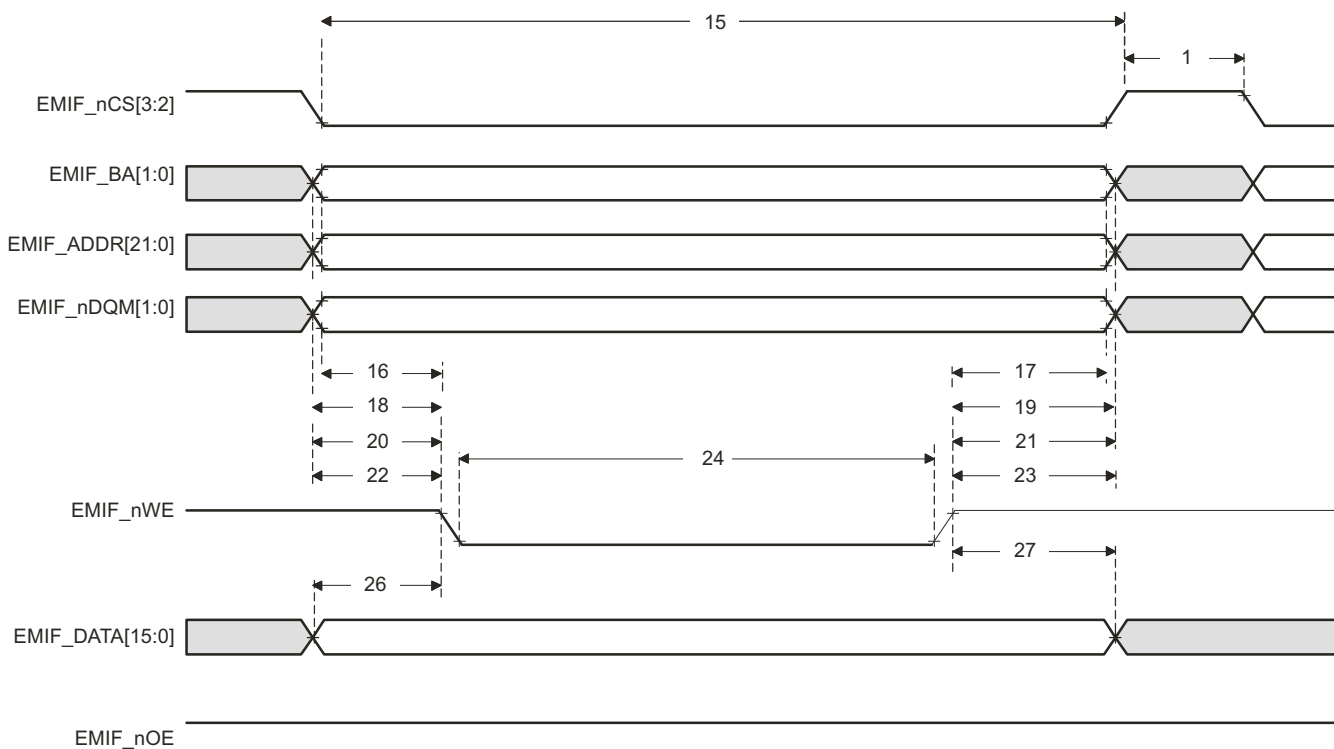
Figure 6-13. Asynchronous Memory Write Timing
